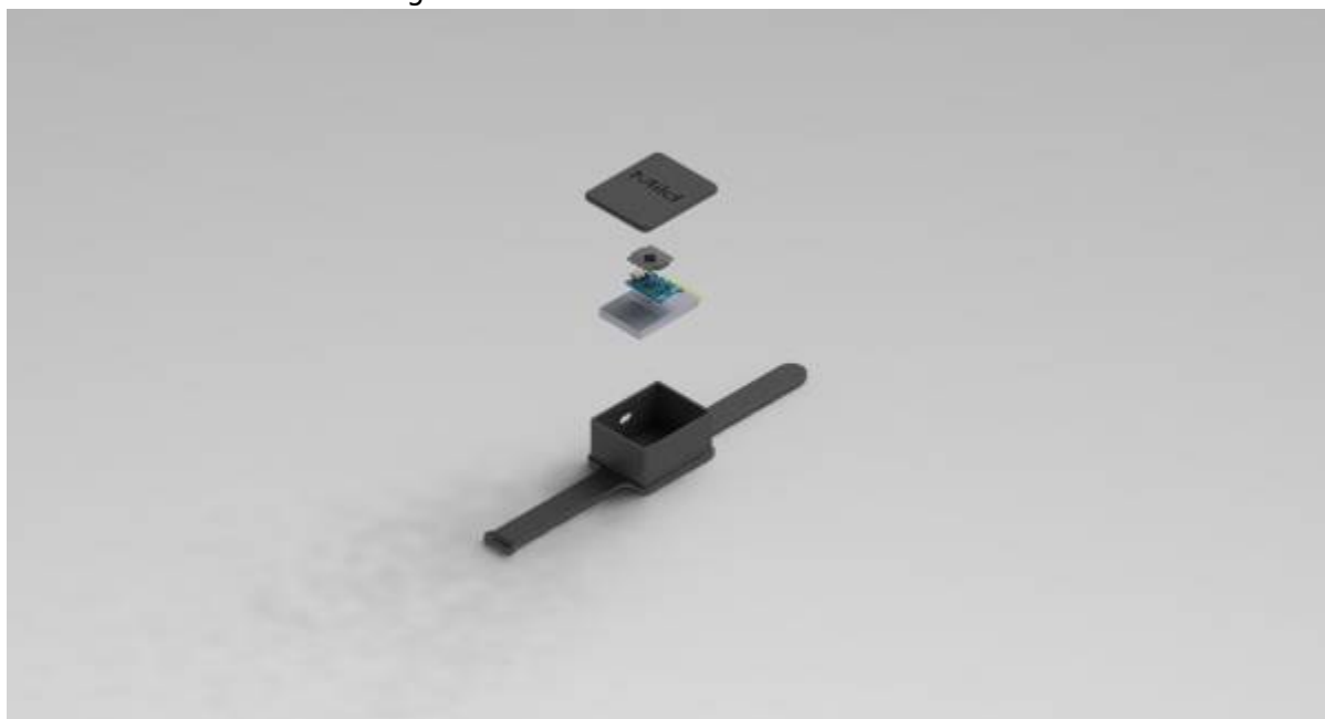
Figure 51: Exploded view of the bracelet
